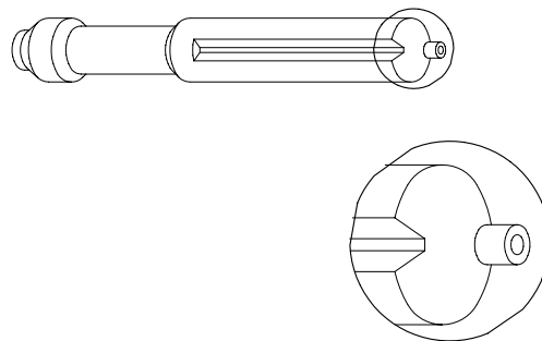
PICK-UP NOZZLE ID=φ0.5, OD=φ1.0 TENRYU, MT-5720
