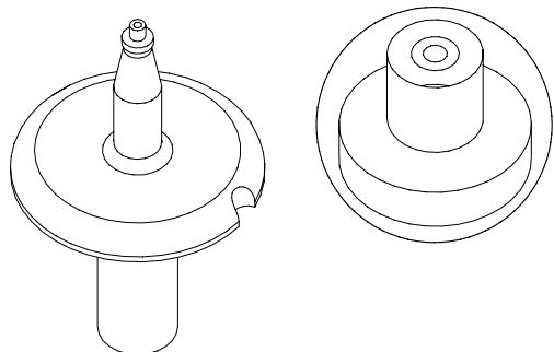
PICK-UP NOZZLE ID=φ0.3, OD=φ1.0
