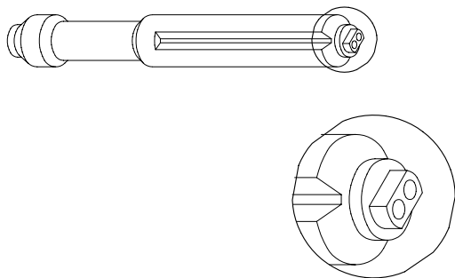
PICK-UP NOZZLE 2 HOLES, ID=φ0.7 PITCH=0.8 TENRYU, MT-5720
