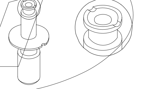
PICK-UP NOZZLE ID=φ1.2 OR φ0.7 TENRYU, MT5300#18
